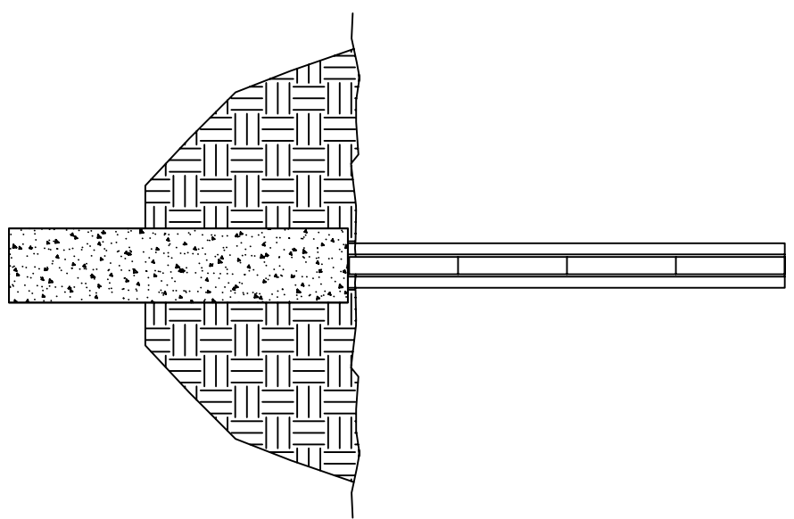
SECTION A STANDARD SOUND WALL 15' MAX POST SPACING
